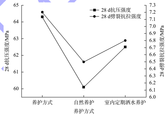
图 5 不同养护条件下试件的强度 Fig. 5 Compressive strength of specimens under different curing conditions
