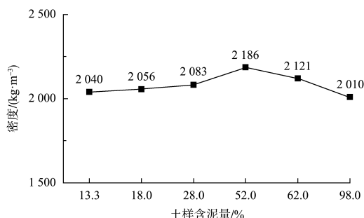
图 2 压制成型下不同含泥量疏浚土块体的密度 Fig. 2 Density of dredged soil blocks with different mud contents under compression molding
