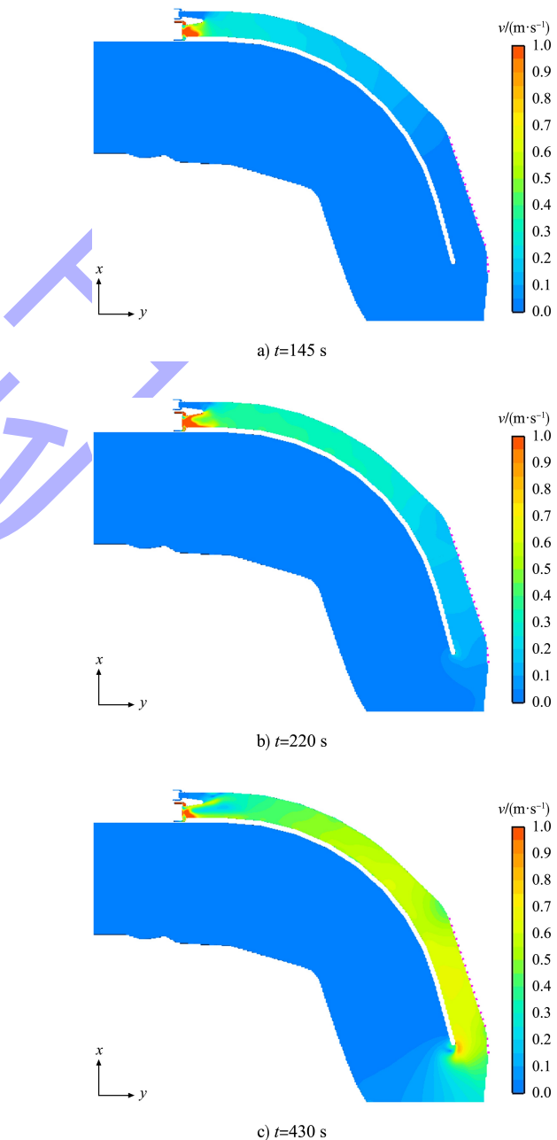
Fig.7 Flow velocity distribution near outlet at each typical moment under 5 min unilateral discharge in left corridor of first-lane ship lock
