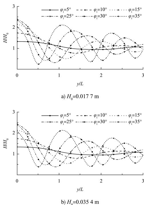
图 9 不同入射角下 x = 5L 处垂直墙面方向比波高分布 Fig. 9 Distribution of relative wave height in direction perpendicular to vertical wall at x = 5L under different incident angles
