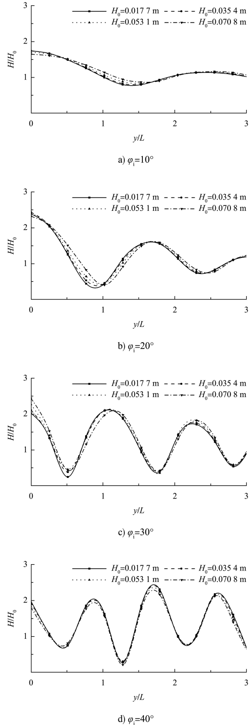
图 12 不同入射波高下 x = 5L 处垂直墙面方向比波高分布 Fig. 12 Distribution of relative wave height in direction perpendicular to vertical wall at x = 5L under different incident wave heights
