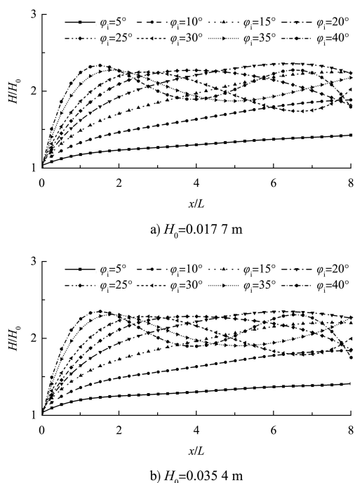
图 6 不同入射波高下 Stem 波沿墙比波高随入射角的变化 Fig. 6 Variation of relative wave height along wall with incident angle for stem waves under different incident wave heights
