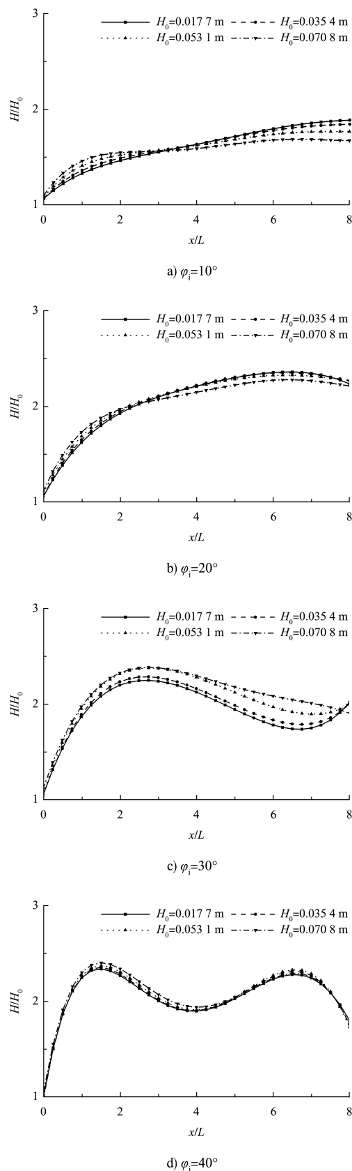
图 10 不同入射角下 Stem 波沿墙比波高随入射波高的变化 Fig. 10 Variation of relative wave height along wall with incident wave height for Stem waves under different incident angles
