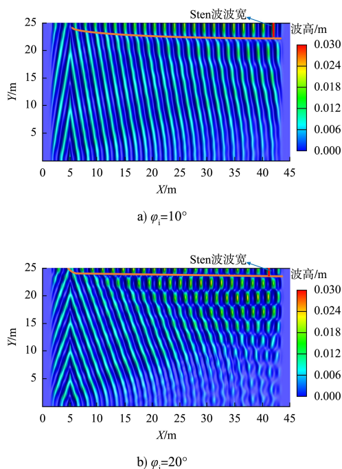
图 8 不同入射角下瞬时自由表面等值线 Fig. 8 Instantaneous free surface contour at different incident angles
